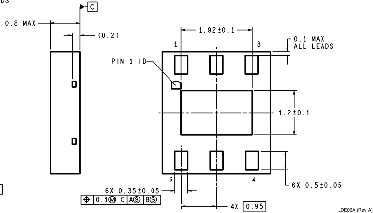
6-Lead LLP Package (LD) NS Package Number LDE06A
